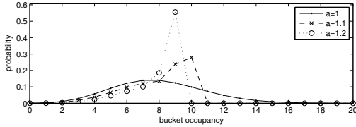
Fig. 2. The probability density function of the distribution P_{LB} over the bucket occupancies. Each distribution P_{LB} induces a lower bound on the balancing cost, given different system constraints. In this figure, we fixed load r = 8 , overflow fraction \gamma = 0 , and used different values of average access rate a .
