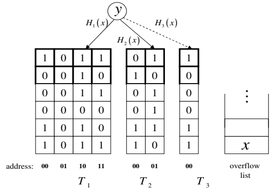
Fig. 1. Illustration of a Bloom Filter implementation using MHT, with three subtables. T_2 only holds elements that did not fit T_1 ; T_3 only holds elements that did not fit T_2 . The upper two bits in each memory block, depicted in bold, are used to count the number of elements.
