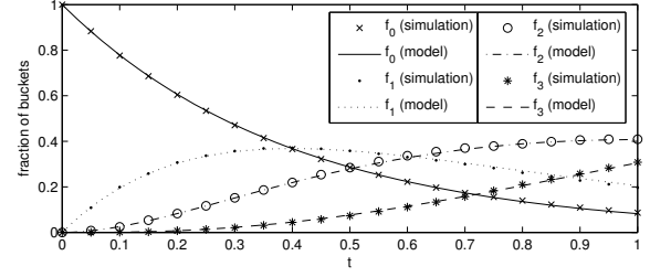
Fig. 5. simulation vs. analytic model for SINGLE with r = 2.5 , p = 0.5 and h = 2
