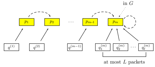
Fig. 2. Outline of mapping \chi . Packet p_1 is admitted to the buffer upon arrival without preempting any packet, and henceforth packet p_{i+1} preempts packet p_i . The mapping \psi along the preemption sequence is depicted by dashed arrows. Such a sequence ends at a packet p_m which is successfully delivered by PQ_\beta . Mapping \phi , depicted by solid arrows, maps at most 1 packet to any packet that is preempted in the sequence, and at most L packets to the last packet of the sequence which is successfully delivered by PQ_\beta . This gives an overall of 2(m-1) + L packets mapped to any single packet successfully delivered by PQ_\beta .
