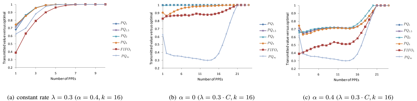
Fig. 8. Performance ratio of online algorithms versus optimal for different values of \alpha , as a function of the number of cores C . In Figure 8(a) the arrival rate is kept constant at \lambda = 0.3 , regardless of the number of cores C . In all other figures the average arrival rate of the simulated traffic for each value of C is proportional to the number of cores (set to \lambda = 0.3 \cdot C ).
