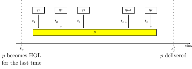
Fig. 6. An outline of the mappings to the HOL packet p in G during the interval H_p = [s_p, s_p^*] . For each i , packet q_i is mapped to p at time t_i .
