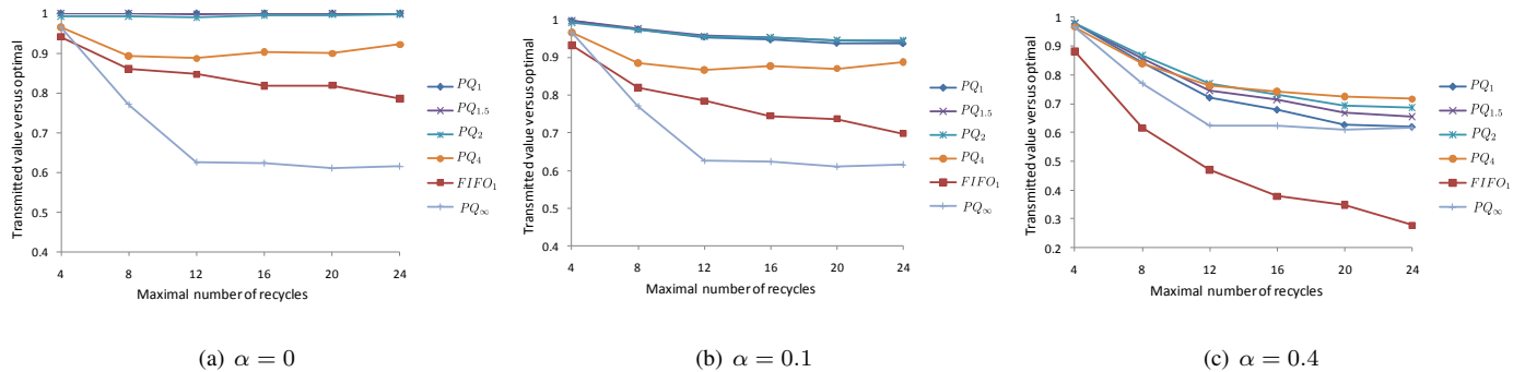
Fig. 7. Performance ratio of online algorithms versus optimal for different values of \alpha , as a function of the maximum number of passes k required by a packet k . The results presented are for a single core (i.e., C = 1 ). The average arrival rate of the simulated traffic for each value of k is fixed to 0.3 (packets per time slot).
