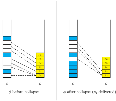
Fig. 4. Outline of a mapping-collapse. Upon the delivery of the HOL packet in G , p_1 , the largest set of live A_1 packets closest to the head of queue in G (but no more than L ) are mapped to the new HOL packet, p_2 , and remaining packets of A_1 in O 's buffer are shifted downwards appropriately. In this example we take L = 3 .
