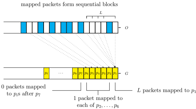
Fig. 5. An example of a mapping which is 6-prefix-full and sequential. Cyan packets are packets that are either in A_2 \cup (O \cap G) or A_1 packets that are no longer alive. Mapped white packets are in A_1 . In the example above, L = 5 .
