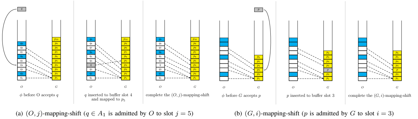
Fig. 3. Outline of mapping-shifts. The new packet is inserted into the corresponding buffer slot, and the mapping is shifted accordingly. Cyan packets are packets that are either in A_2 \cup (O \cap G) , or packets in A_1 that are no longer alive. White packets are live A_1 packets, which might be affected by changes in the mappings. In both examples L = 3 .
