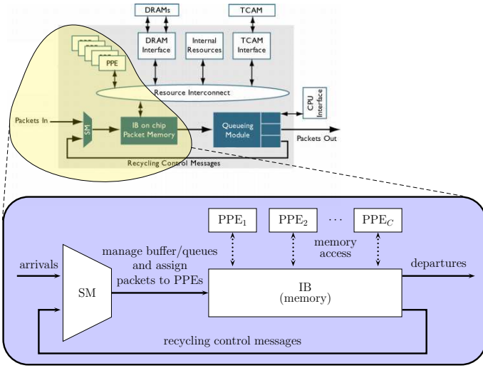
Fig. 1. An outline of the architecture model, as an abstraction of a standard Multipass NP Architecture (see, e.g. [33]).
